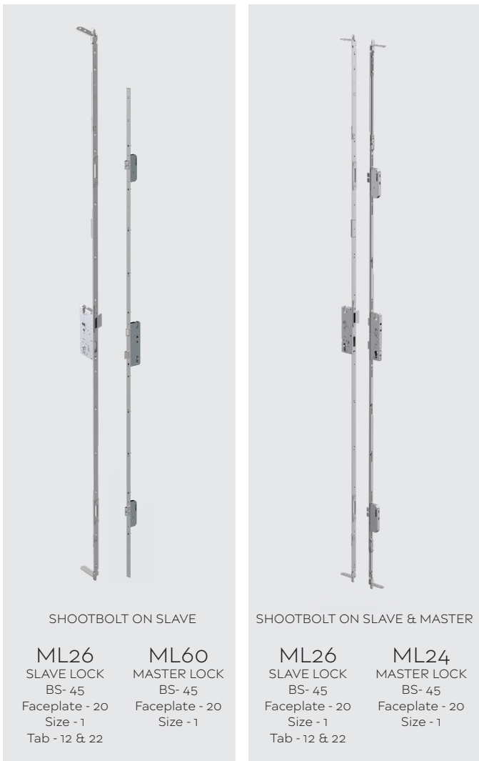
DOUBLE DOORS - TWIN HANDLE
