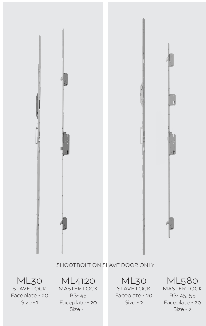
DOUBLE DOORS - SLAM SHUT
